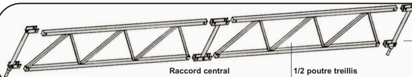
Raccord central Ref. 0351 Poids: 3 kg
